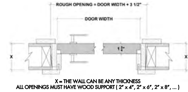
Standard Installation Flush with Drywall Installation
