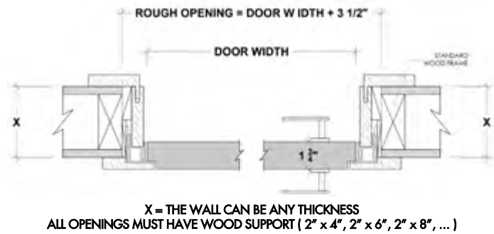
Standard Installation Flush with Drywall Installation
