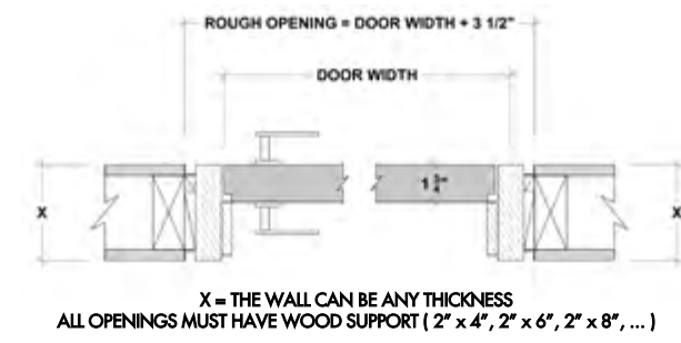
Standard Installation Jamb Proud of the wall Installation
